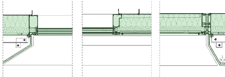
Zone 1.0 - Typical Mullion Detail
