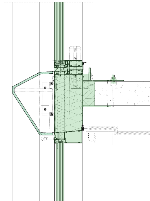
Zone 1.0 - Floor Edge Detail
