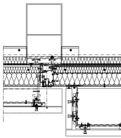
EWS03 - Typical horizontal section at spandrel (left&right)
