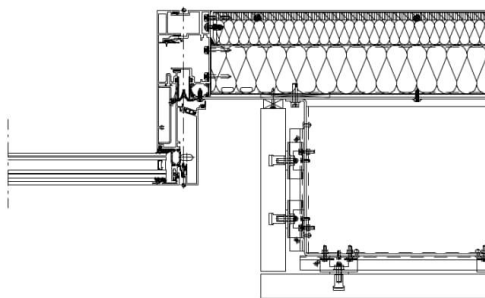
EWS03 - Typical horizontal section at vision (left&right)
