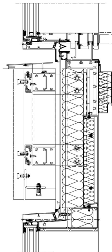
EWS03 - Typical vertical section at stack joint
