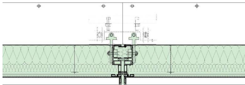
EWS 101 – Typical mullion (spandrel)
