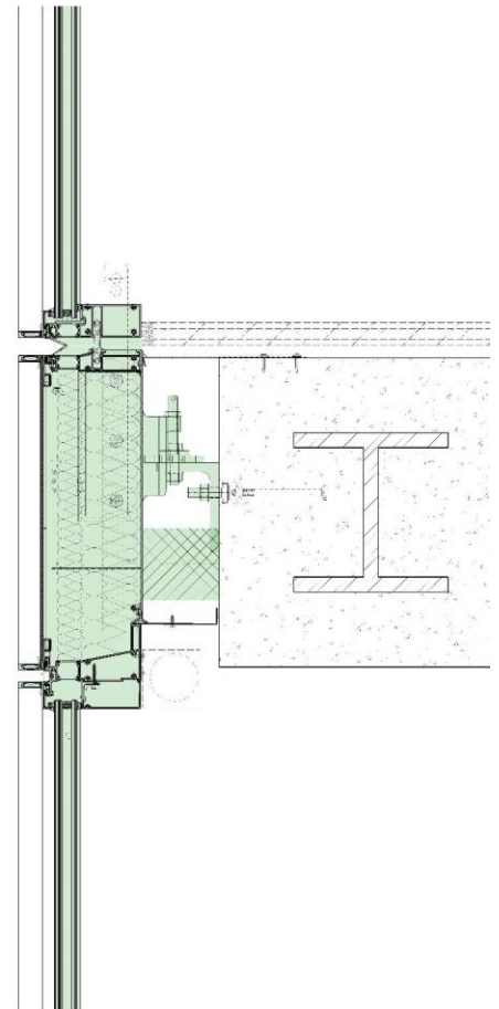
EWS 101 – Typical floor edge detail
