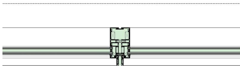
EWS 101 – Typical mullion (glazing)
