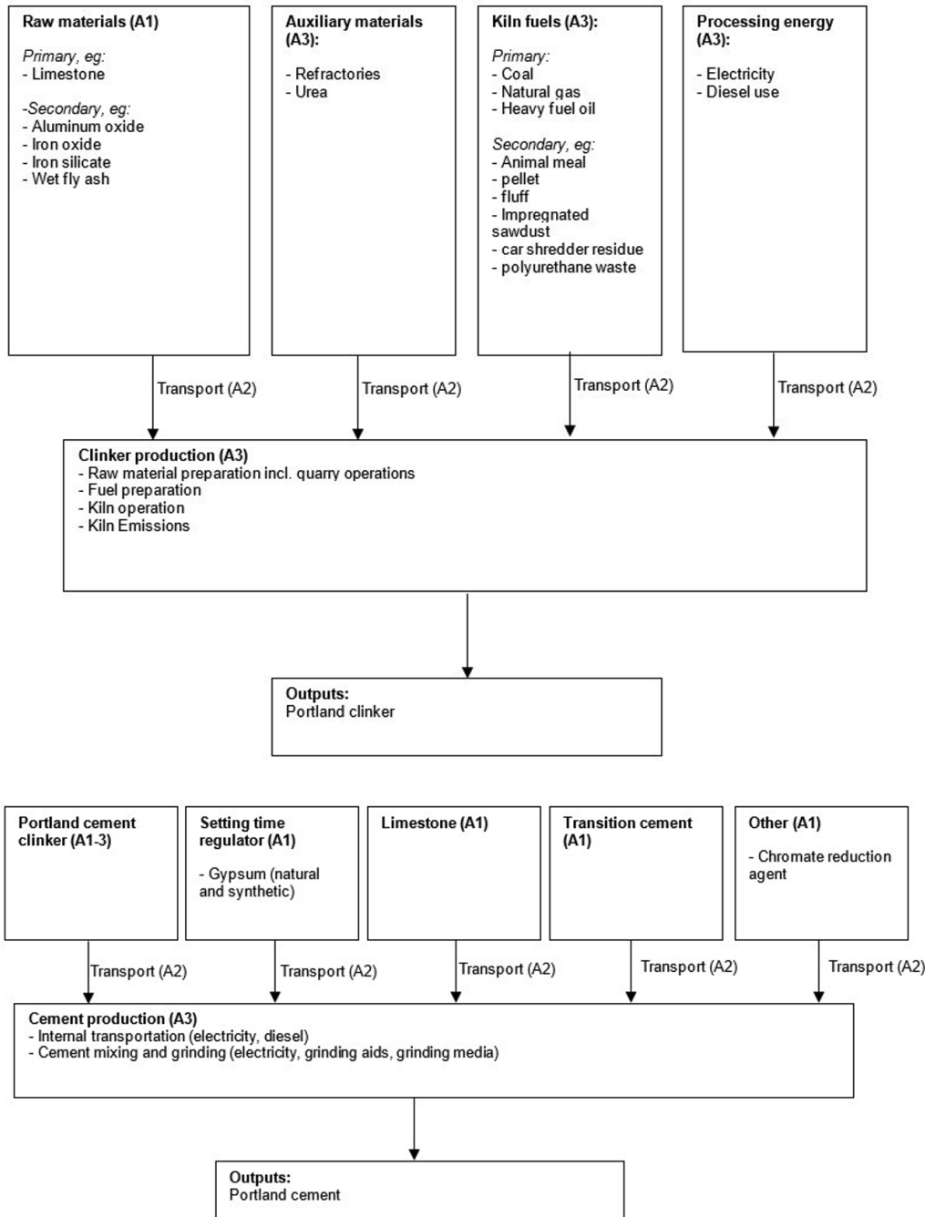
LCA process diagram according to EN 15804 (7.2.1)
