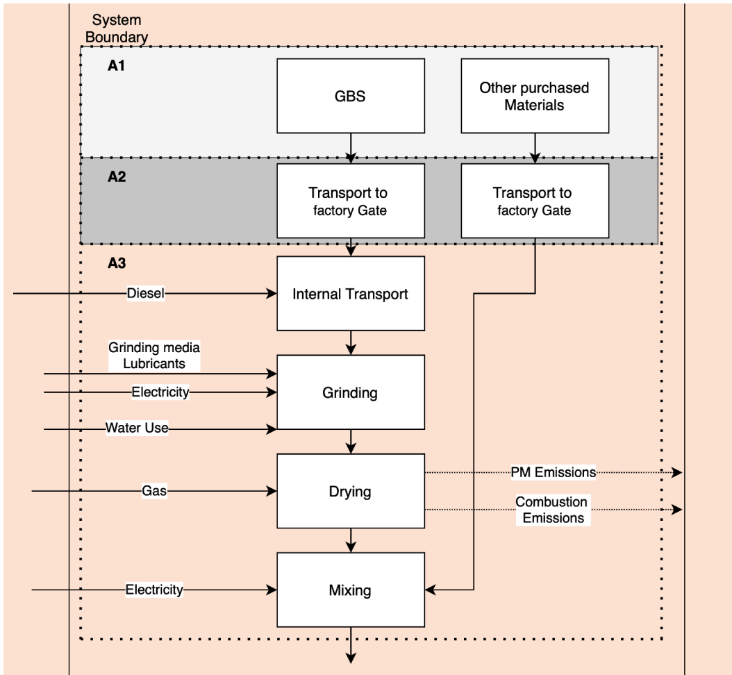
LCA process diagram according to EN 15804 (7.2.1)
