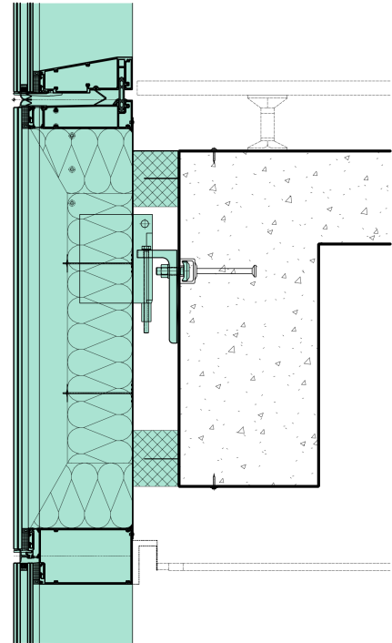
EWS2G - Typical floor edge detail
