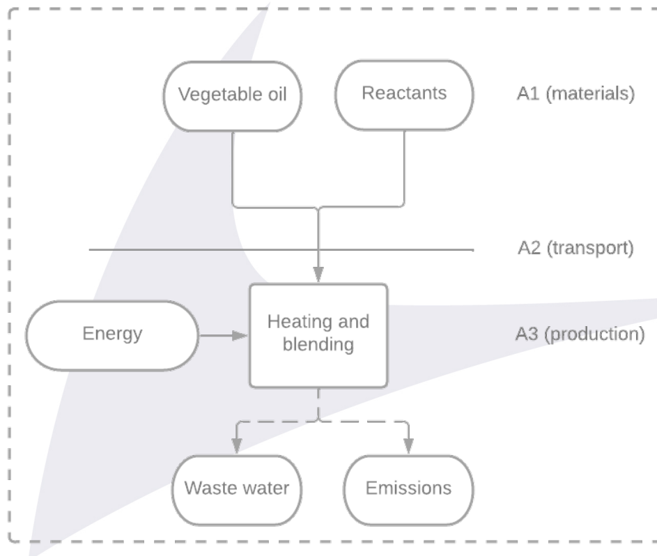
LCA process diagram according to EN 15804 (7.2.1)
