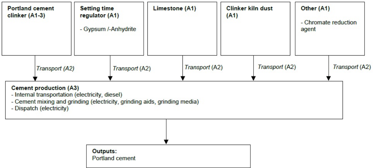
Figure 2.1b Schematic overview of the production of Portland cements
